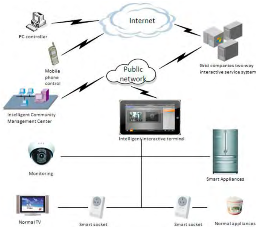
Figure 3.1. Structure of the system for electrical service of a smart home
