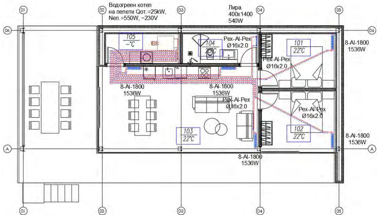
Figure 1.2. Piping and heat consumers
