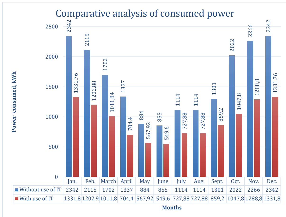
Figure 4.6. Comparative analysis of consumed electricity
