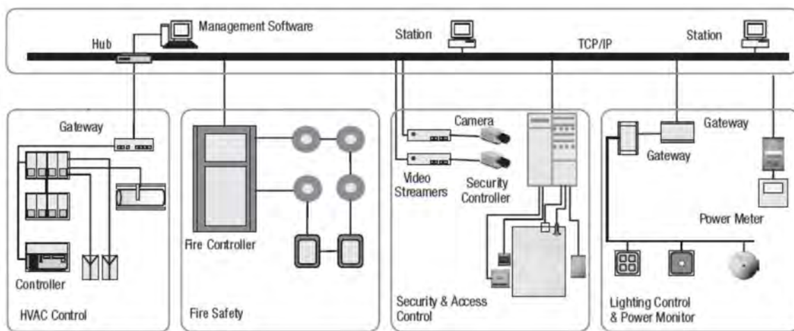
Figure 2.3. Integrated intelligent building system
