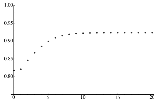
Figure 2: The orthotropic problem, \epsilon = 2^{-t} , t \in \{0, 1, \dots, 20\} : An estimated convergence factor according to (16) plotted against t .
