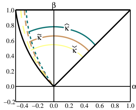
Figure 1b: \{\alpha, \beta\} : \gamma_E^2 \leq \frac{8}{9} .
