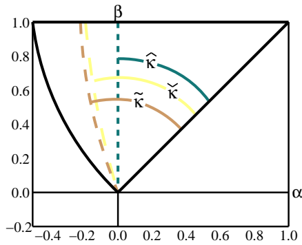
Figure 1a: \{\alpha, \beta\} : \gamma_E^2 \leq \frac{3}{4} .
