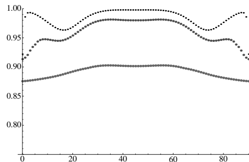
Figure 3: The rotated diffusion problem, \epsilon \in \{10^{-1}, 10^{-2}, 10^{-3}\} , \theta \in \{0^\circ, 1^\circ, \dots, 90^\circ\} : An estimated convergence factor according to (16), plotted against \theta .
